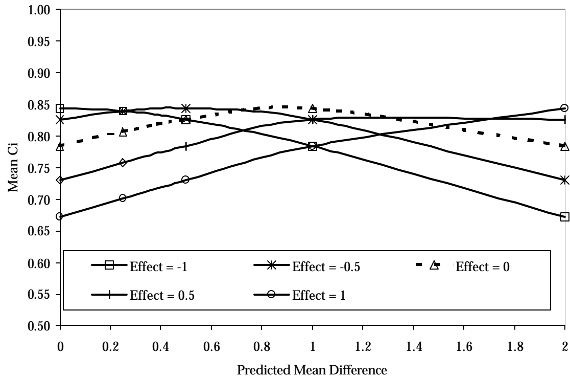
Figure 7. Mean Value of C_i by Theory Prediction and Effect of Extraneous Variable. True Mean Difference = 1.0.
