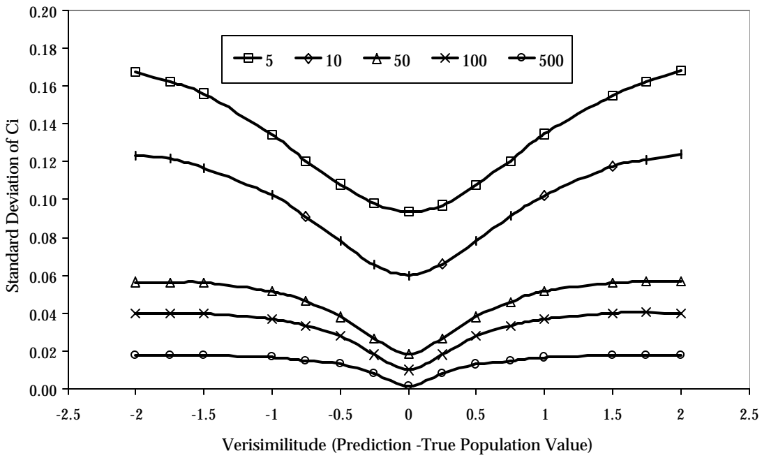
Figure 4. Standard Deviation of Meehl's C_i by Verisimilitude and Sample Size.
