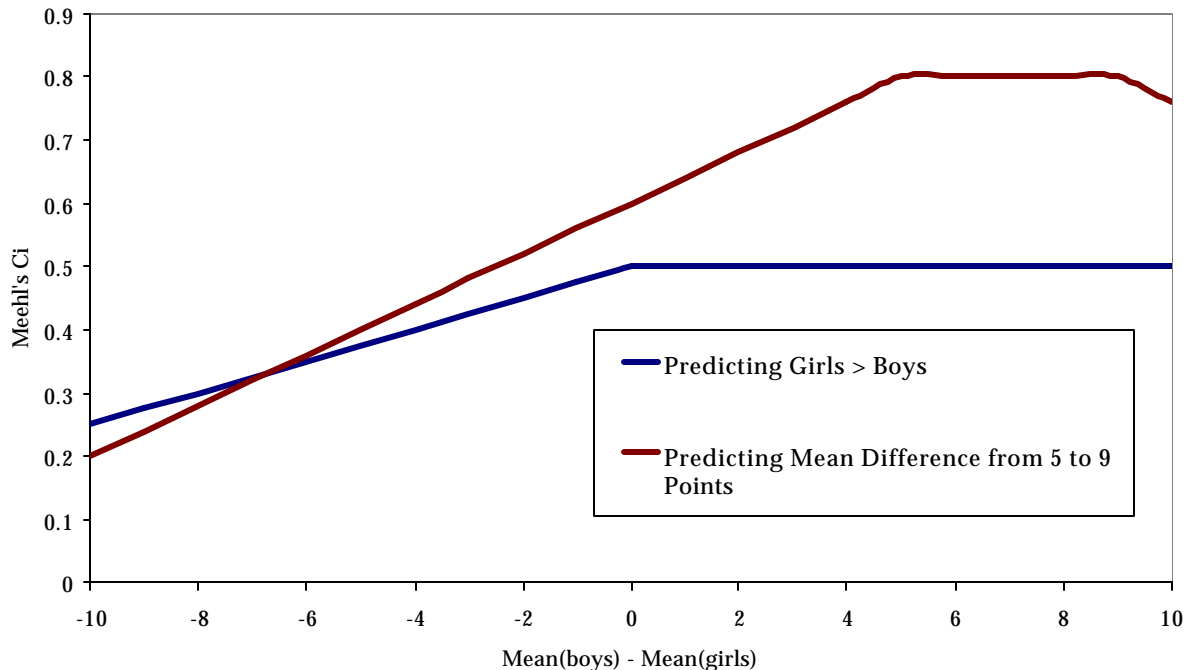
Figure 1. Meehl's C_i by Observed Mean Difference
