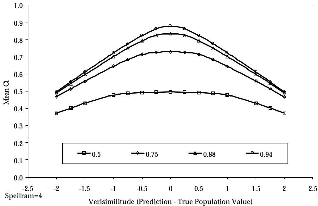
Figure 2. Mean Value of Meehl's C_i by Intolerance and Verisimilitude.
