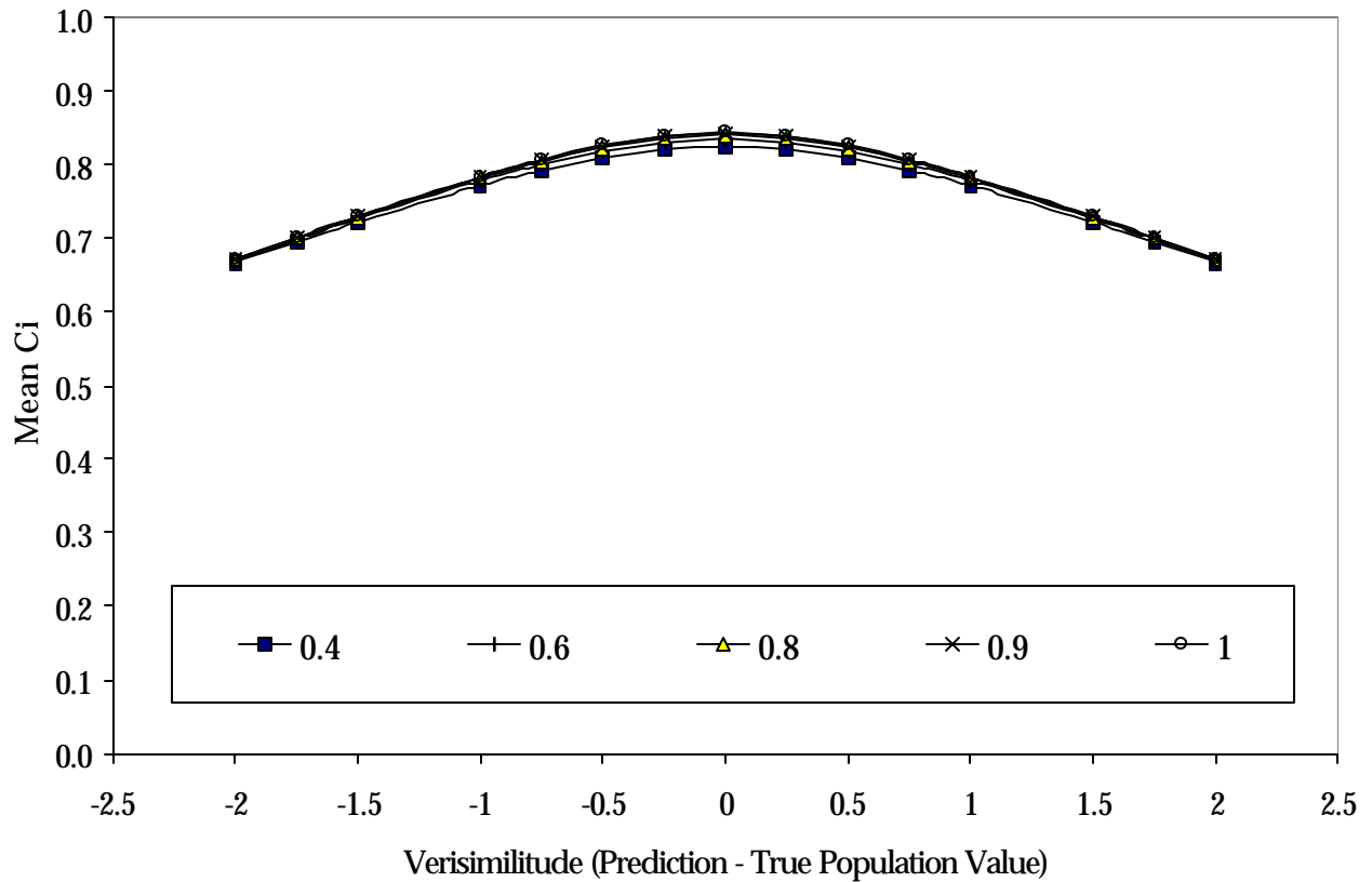
Figure 5. Mean Value of Meehl's C_i by Verisimilitude and Reliability.
