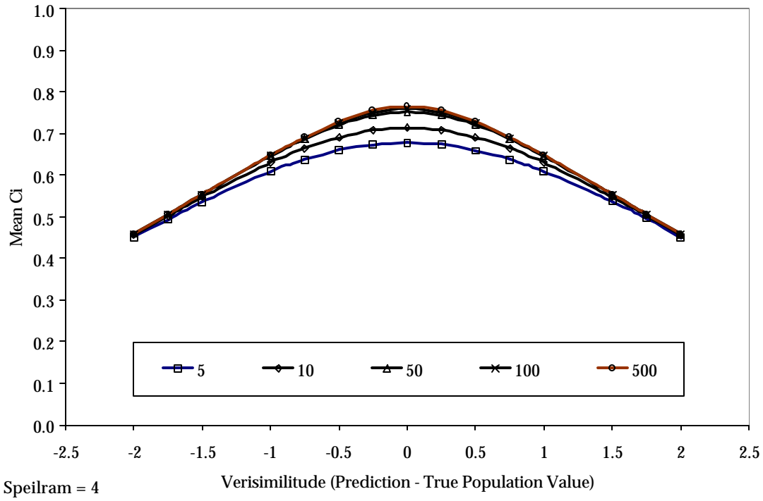
Figure 3. Meehl's C_i by Verisimilitude and Sample Size.
