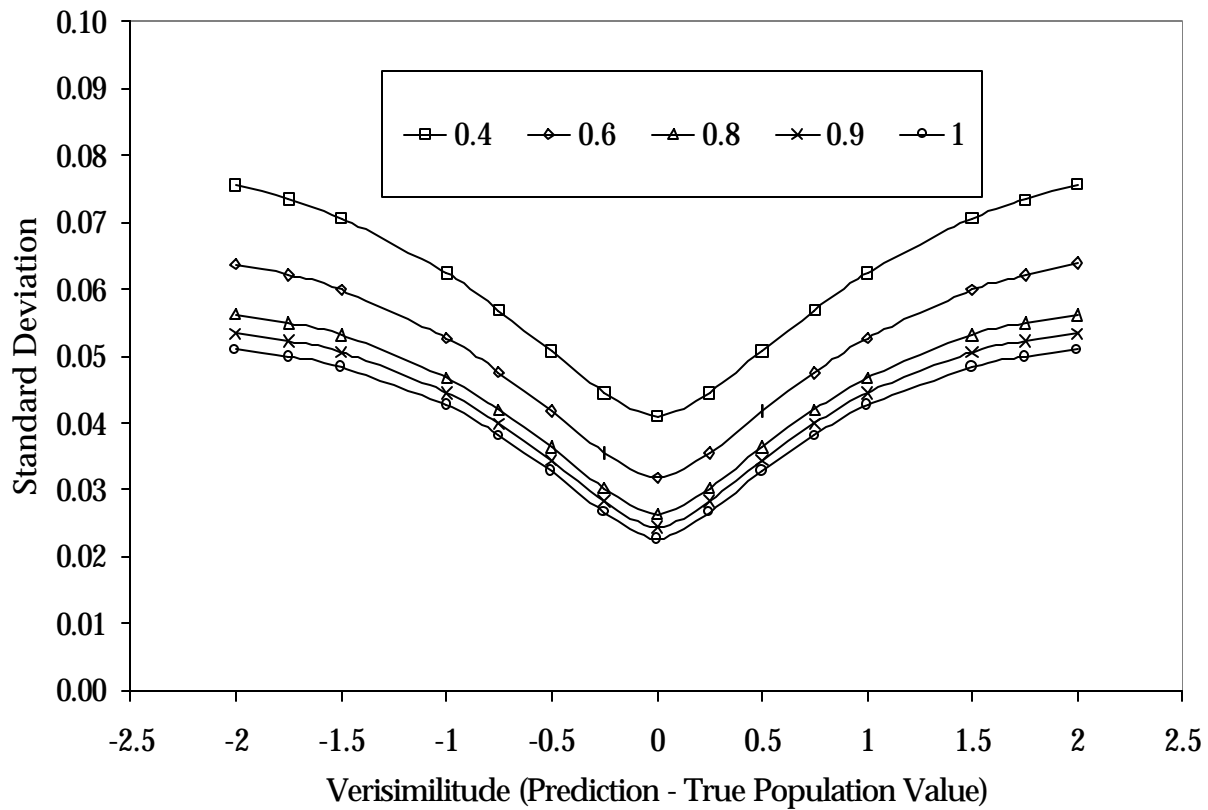
Figure 6. Standard Deviation of Meehl's C_i by Verisimilitude and Reliability.
