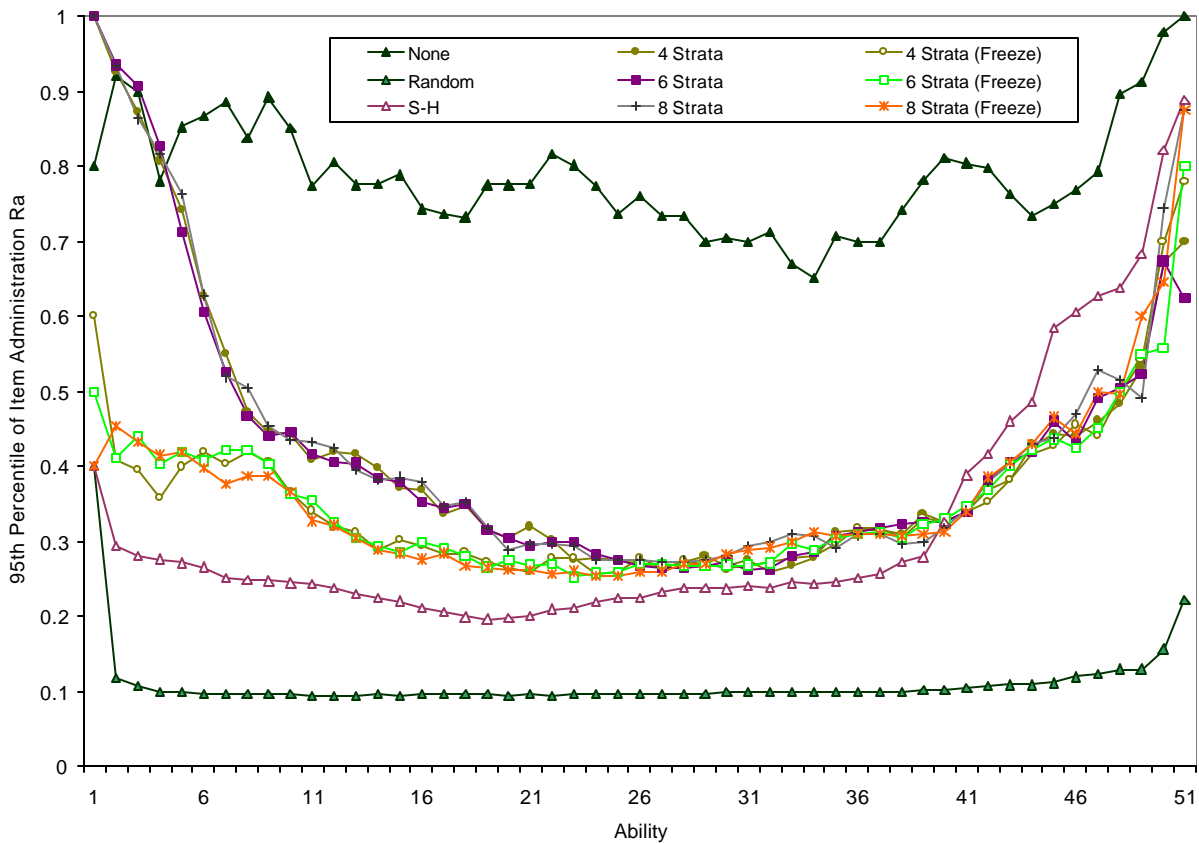
Figure 3a. 95th Percentiles of Conditional Exposure Distributions (Target Maximum Exposure Rate = 0.15)
