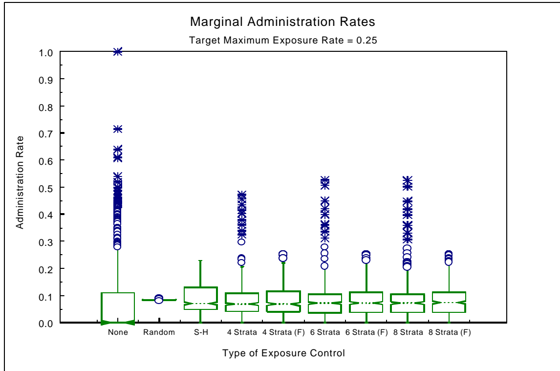
Figure 1b. Marginal Administration Rates by Type of Exposure Control
